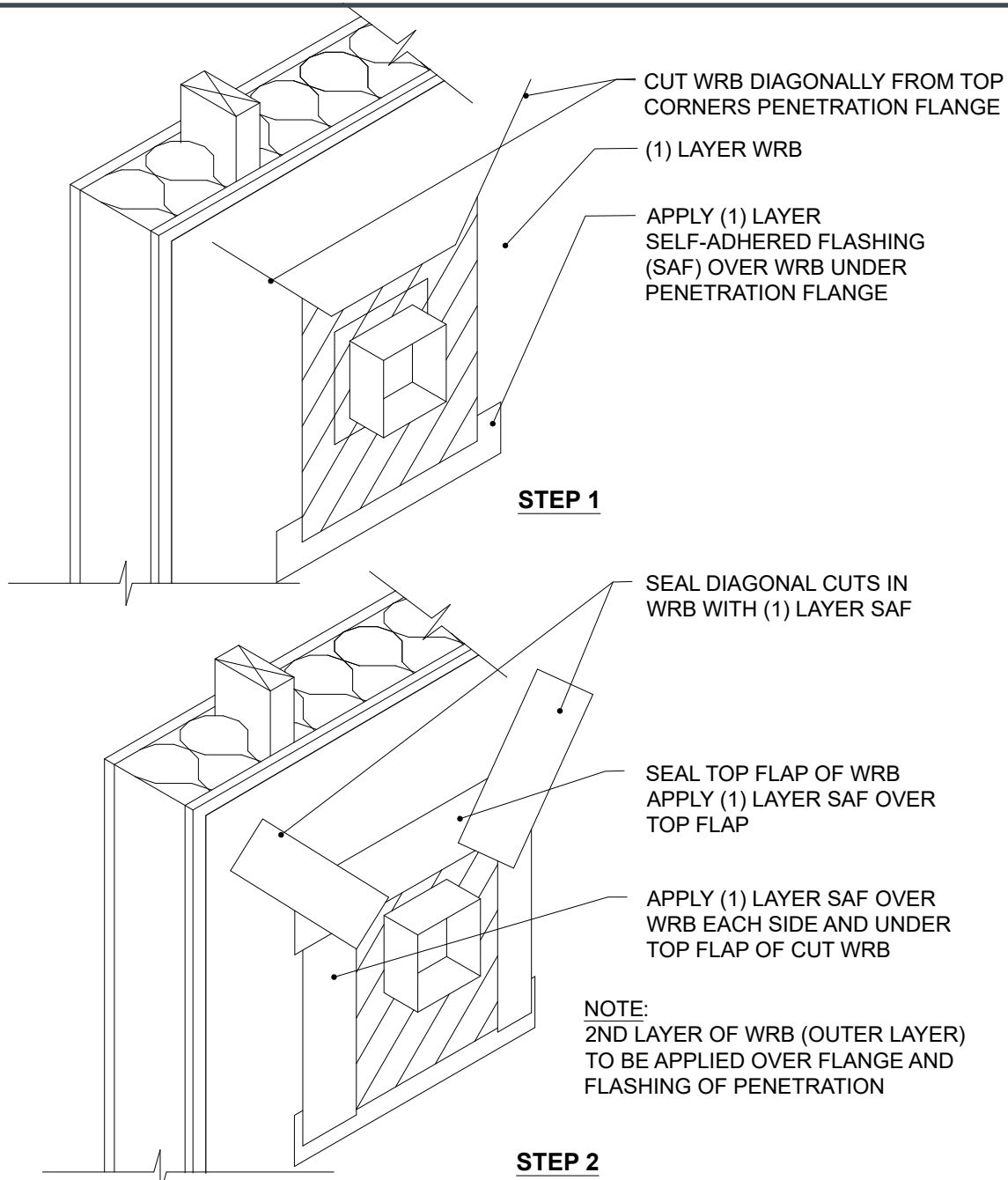
Figure 28. Penetration, Flanged
