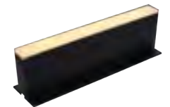
TS-HPL-9 - 12V / 2.5W LED Paver Light 9" x 3/4" x 2 3/8"
