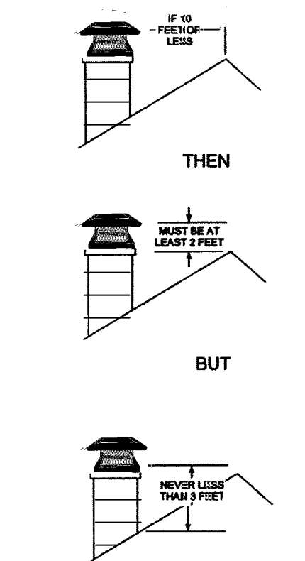
Figure 4. Chimney Height
